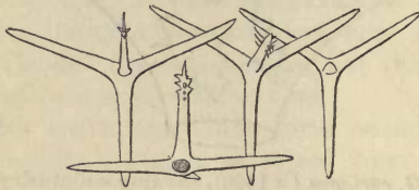
FIG. 7.—Three-spined quadriradiate spicules of A. cerebrum in perspective; the interior of the distant rays in one spicule indicated by shading. The fourth spicule is drawn from above; it is not spined, but the apical ray shows a distinctly triangular section. All \times 260 .
